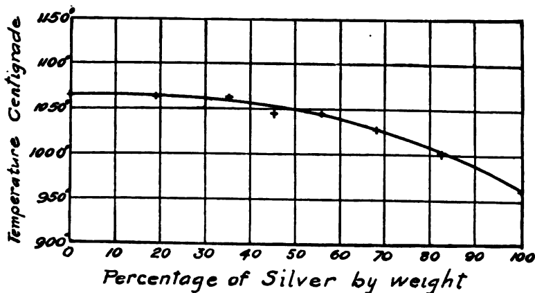
Fig. 29. Freezing-point Curve of Silver-gold Alloys.
